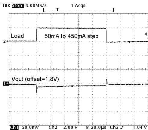
Load Transient Response (50mA to 500mA)
