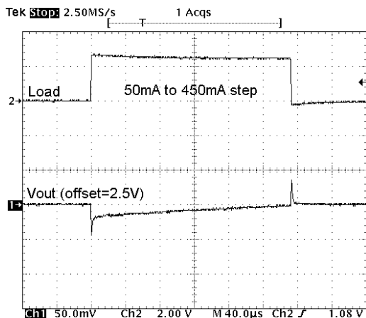
Load Transient Response (50mA to 450mA)
